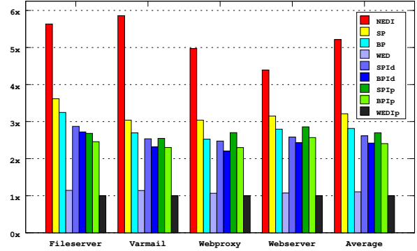
Fig. 10: Filebench results, normalized to NED I_p .
