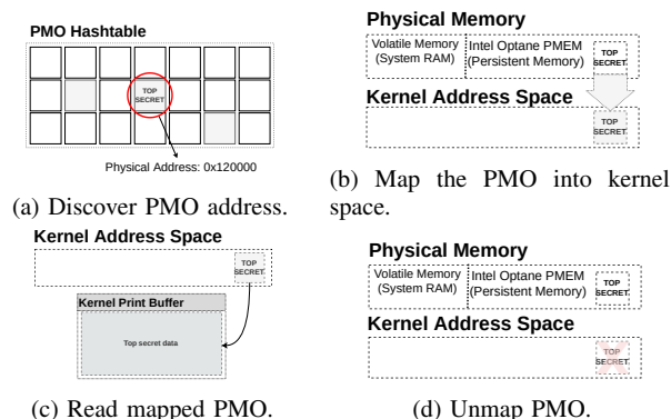
Fig. 2: Steps of PMO example attack, from [13].
