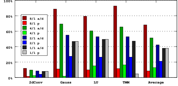
Fig. 9: Pages accessed between attach/detach calls and psyncs , by benchmark and attach/detach size. a/d is the average number of dirtied pages between attach/detach calls, while p is the average number of dirtied pages between psyncs .
