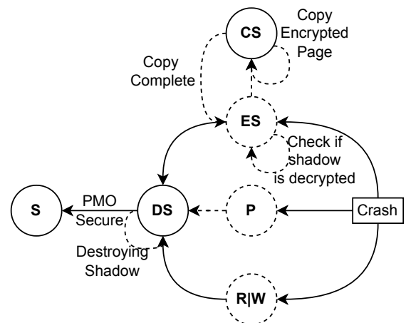
Fig. 5: State transitions for the crash handler
