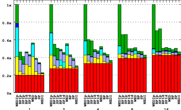
Fig. 7: Average execution time for all the microbenchmarks with different attach sizes, normalized to WED I_p
